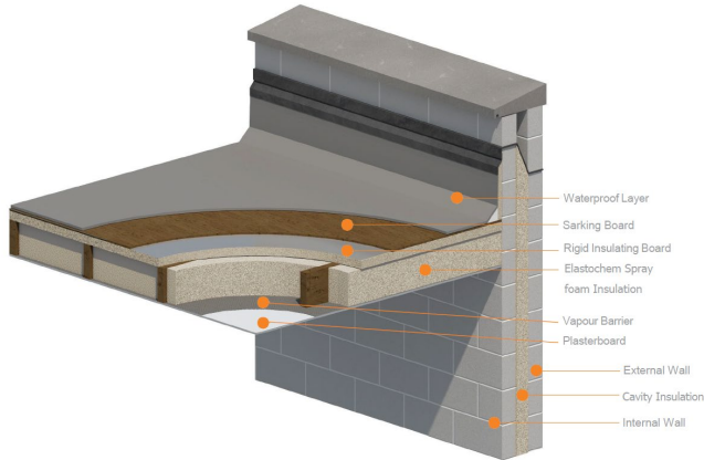
Diagram 1 - Details of typical timber-framed flat roof
