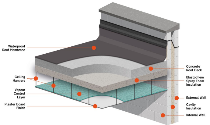
Diagram 2 - Details of typical concrete flat roof
