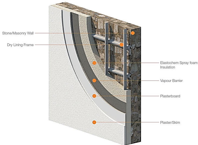
Diagram 1 - Detail of external masonry wall (with dry-lining frame)
