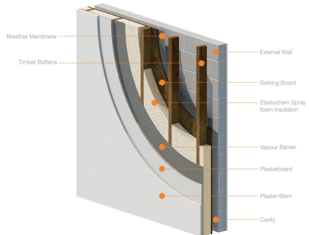
Diagram 2 - Detail of external masonry wall with sheathed timber frame
